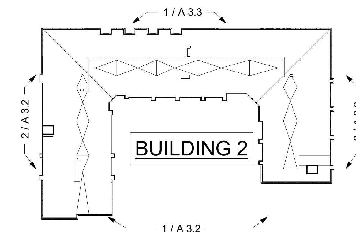
3 BUILDING 2 ELEVATION KEY PLAN 1" = 60'-0"
