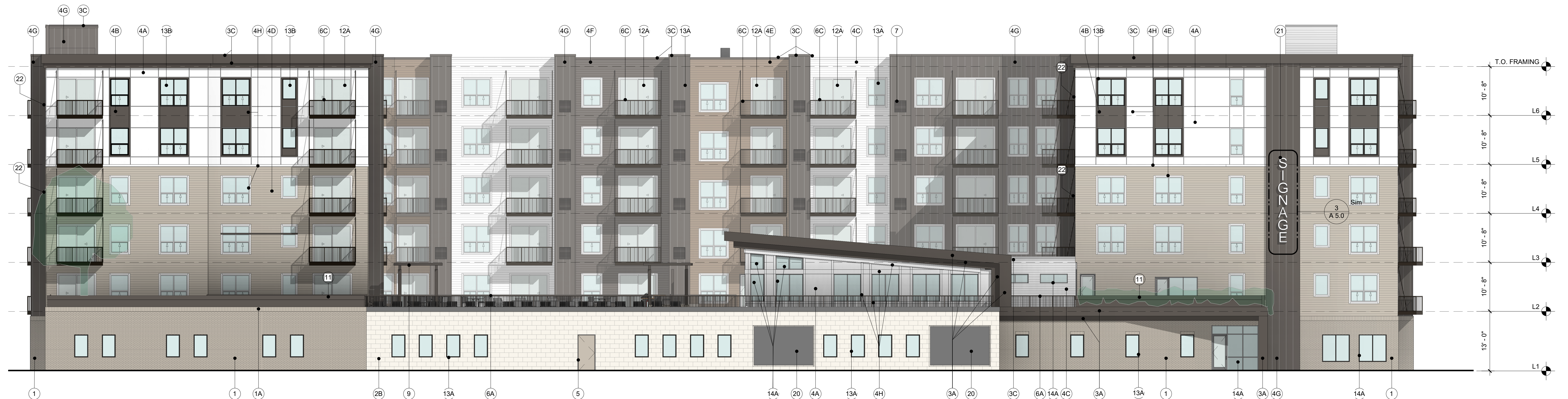
1 PHASE 2 - SOUTH ELEVATION 3/32" = 1'-0"
