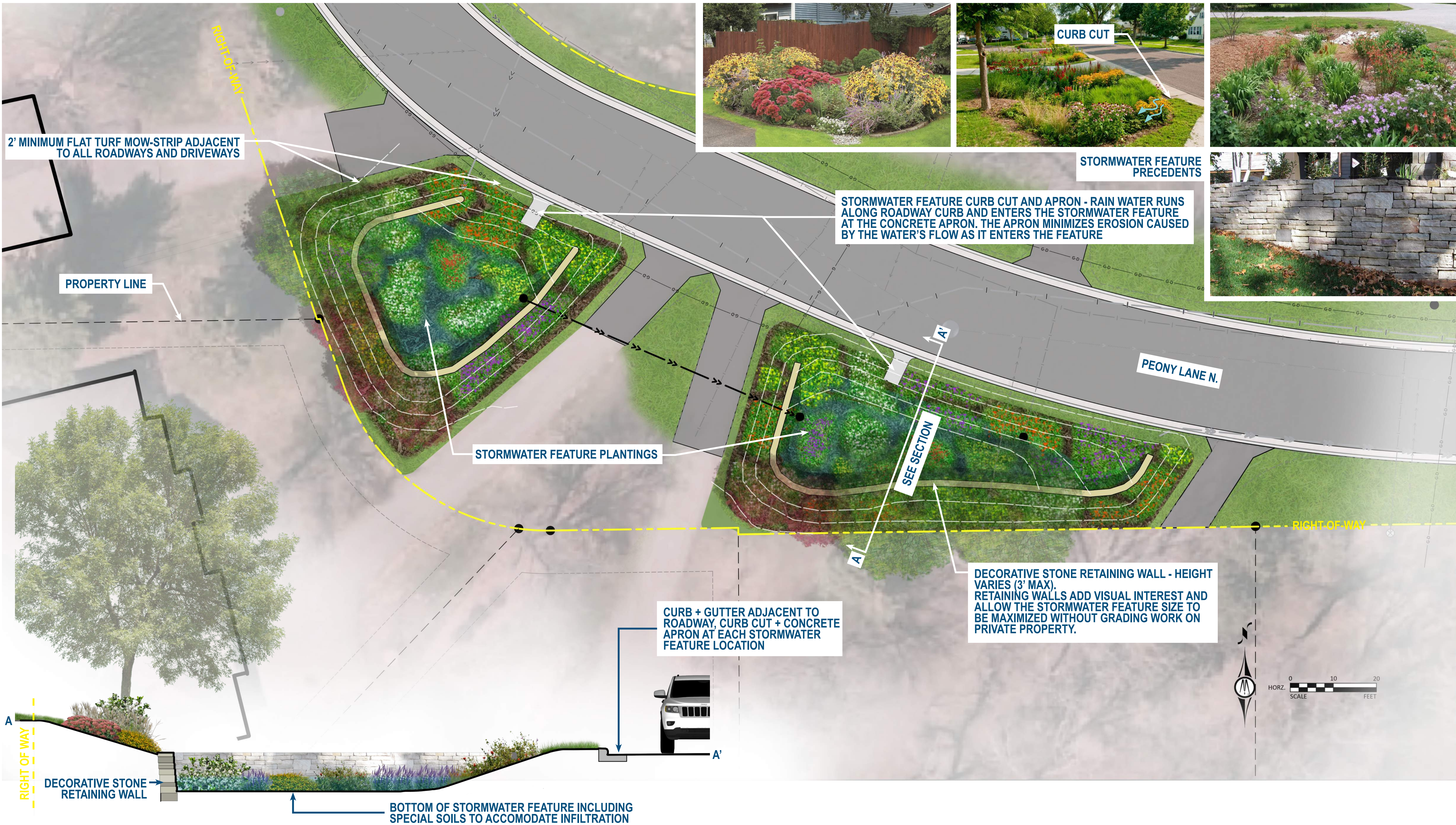
TYPICAL STORMWATER FEATURE SECTION
